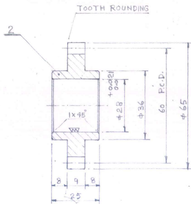
SPUR GEAR
