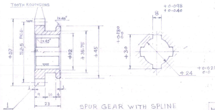
SPUR GEAR WITH SPLINE
