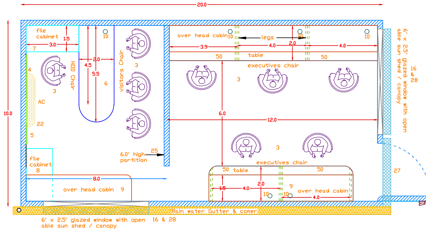
EXECUTIVE IN CHARGE / HOD BUNK HOUSE - 20' X 10' X 10' - B TYPE BUNK HOUSE.
