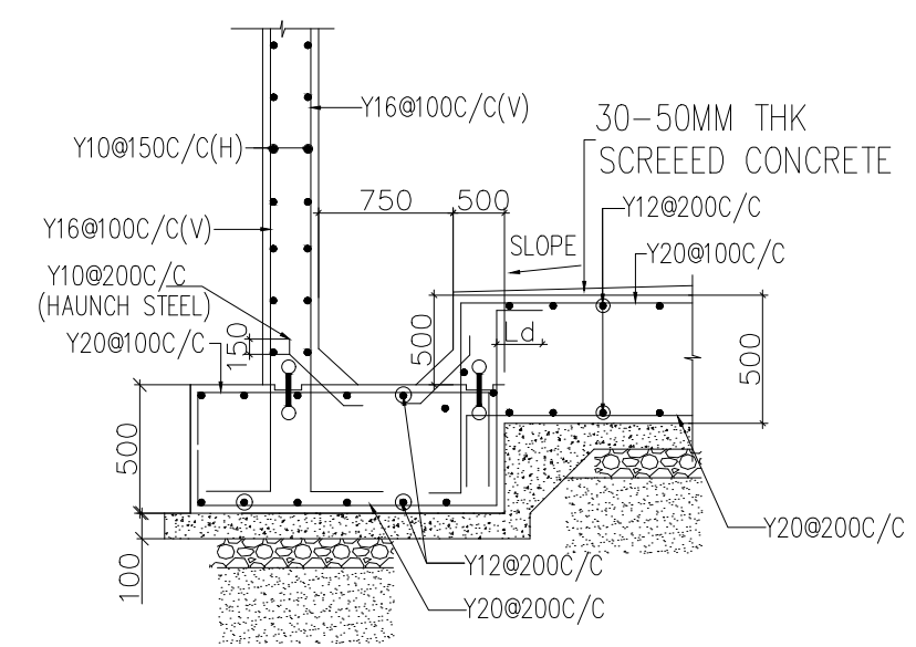
SILT PIT DETAIL SECTION E-E
