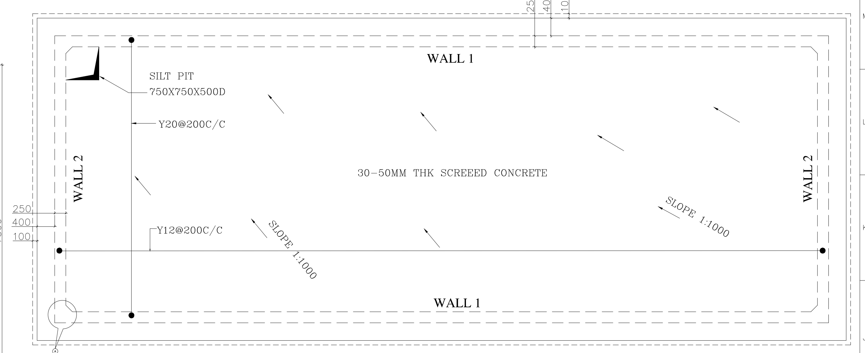
BASE SLAB BOTTOM REINFORCEMENT DETAILS SLAB THICKNESS = 500MM (PLAN)
