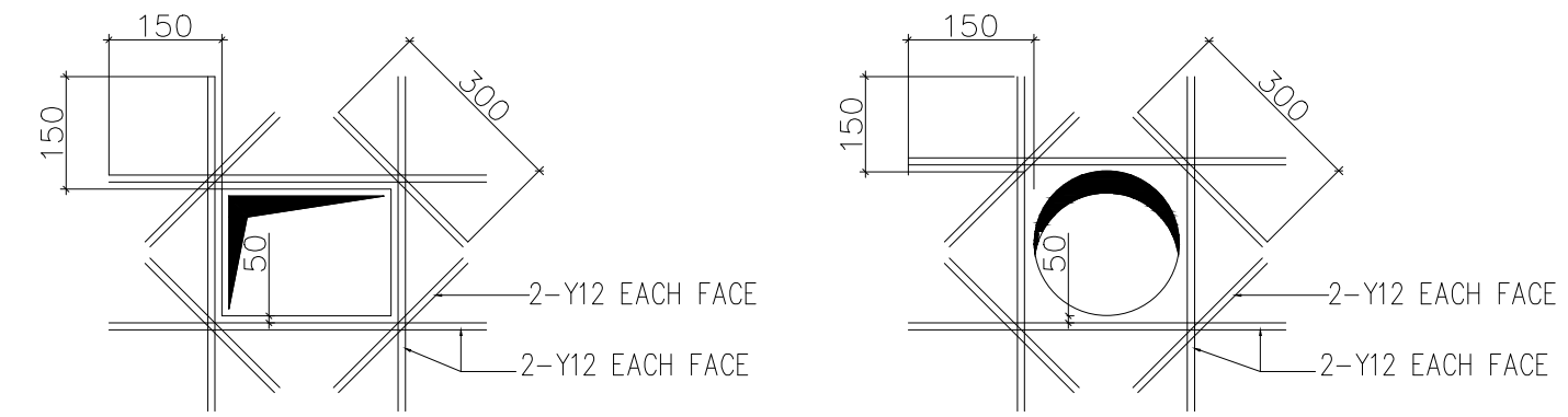
TYPICAL OPENING DETAIL
