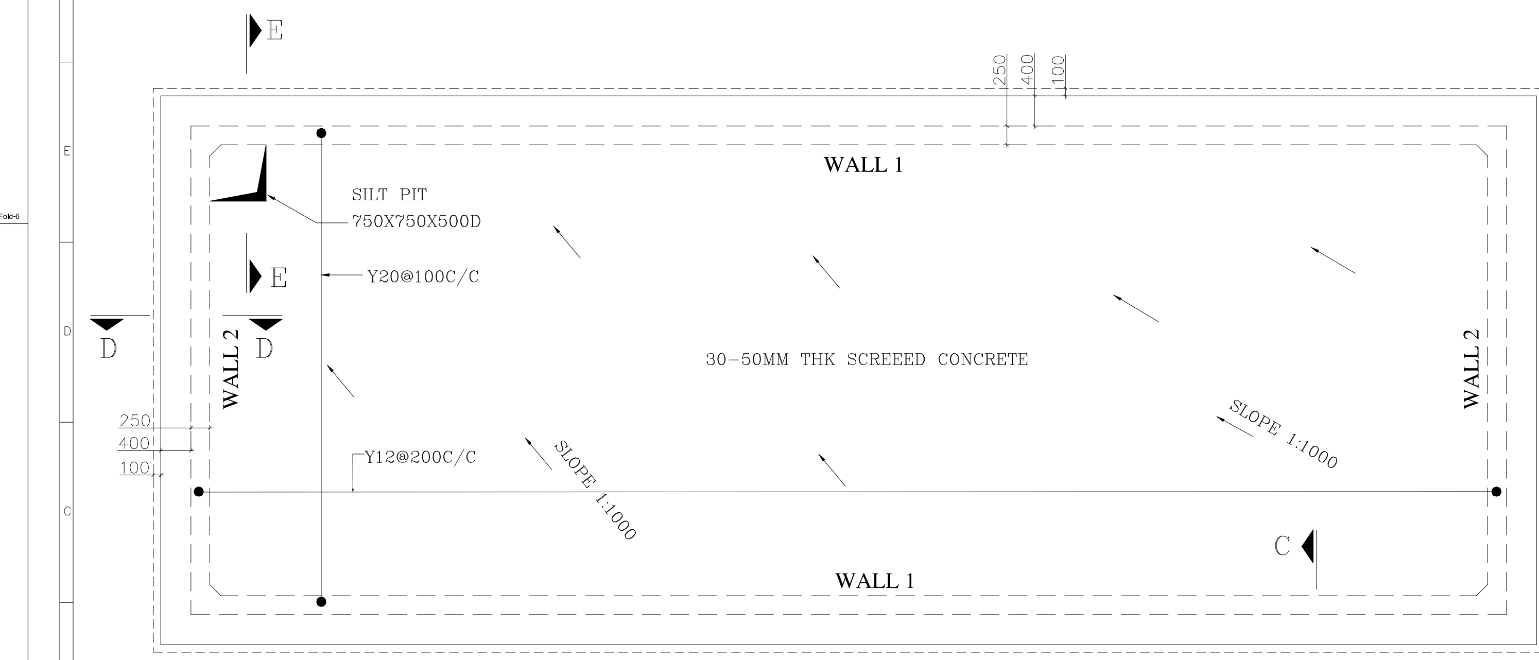
BASE SLAB TOP REINFORCEMENT DETAILS SLAB THICKNESS = 500MM (PLAN)
