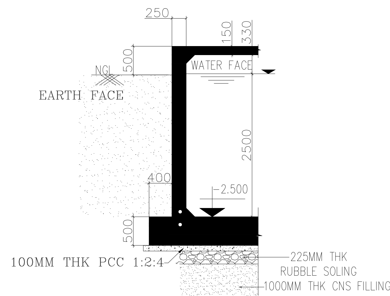
CONCRETE DIMENSION WALL-1&2 DETAILS
