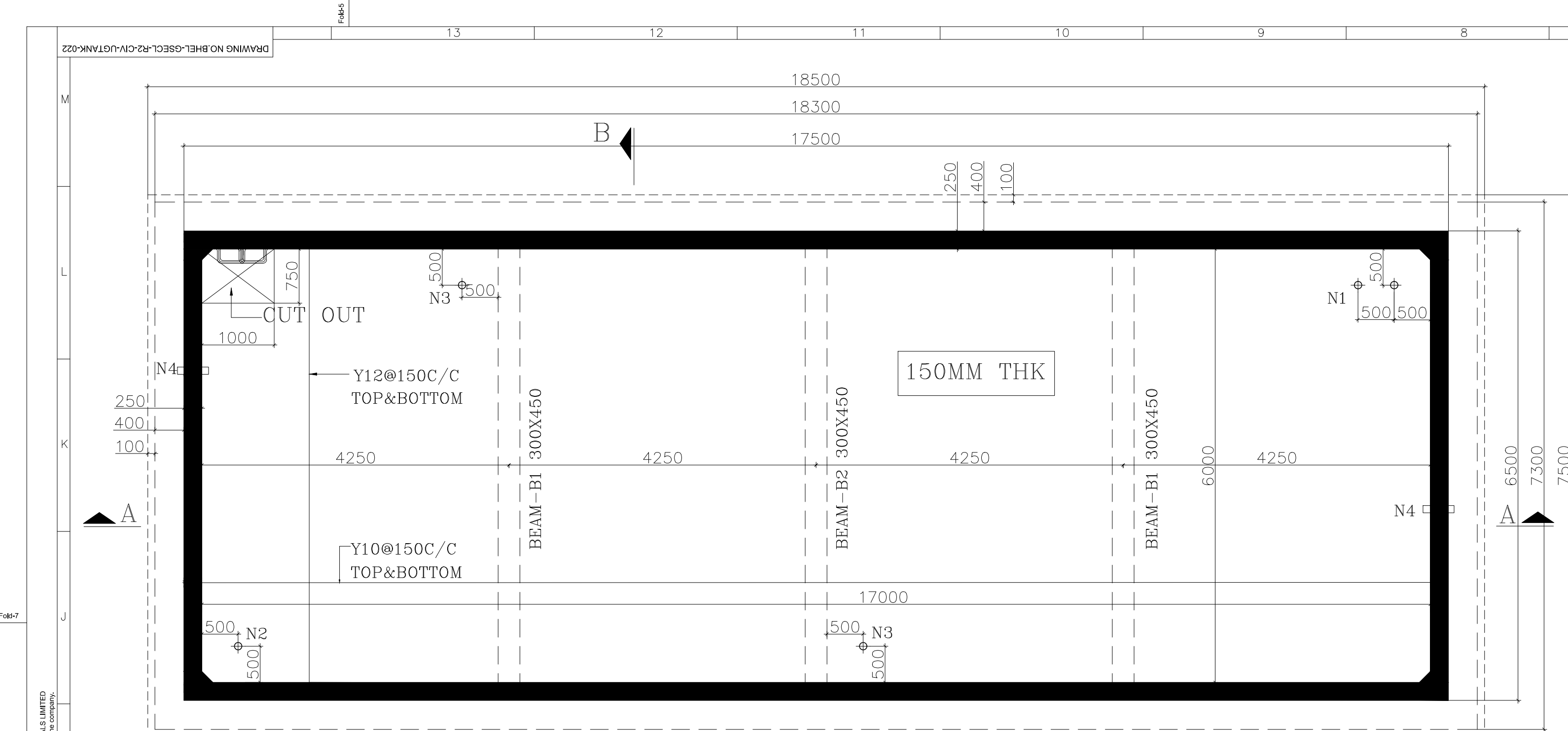
TOP SLAB PLAN @ +0.500 LVL (TOC) T=150MM UNLESS SPECIFIED
