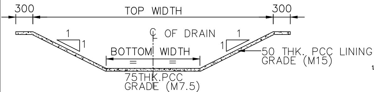
TYPICAL DETAIL OF PERIPHERAL DRAIN / INTERNAL DRAIN
