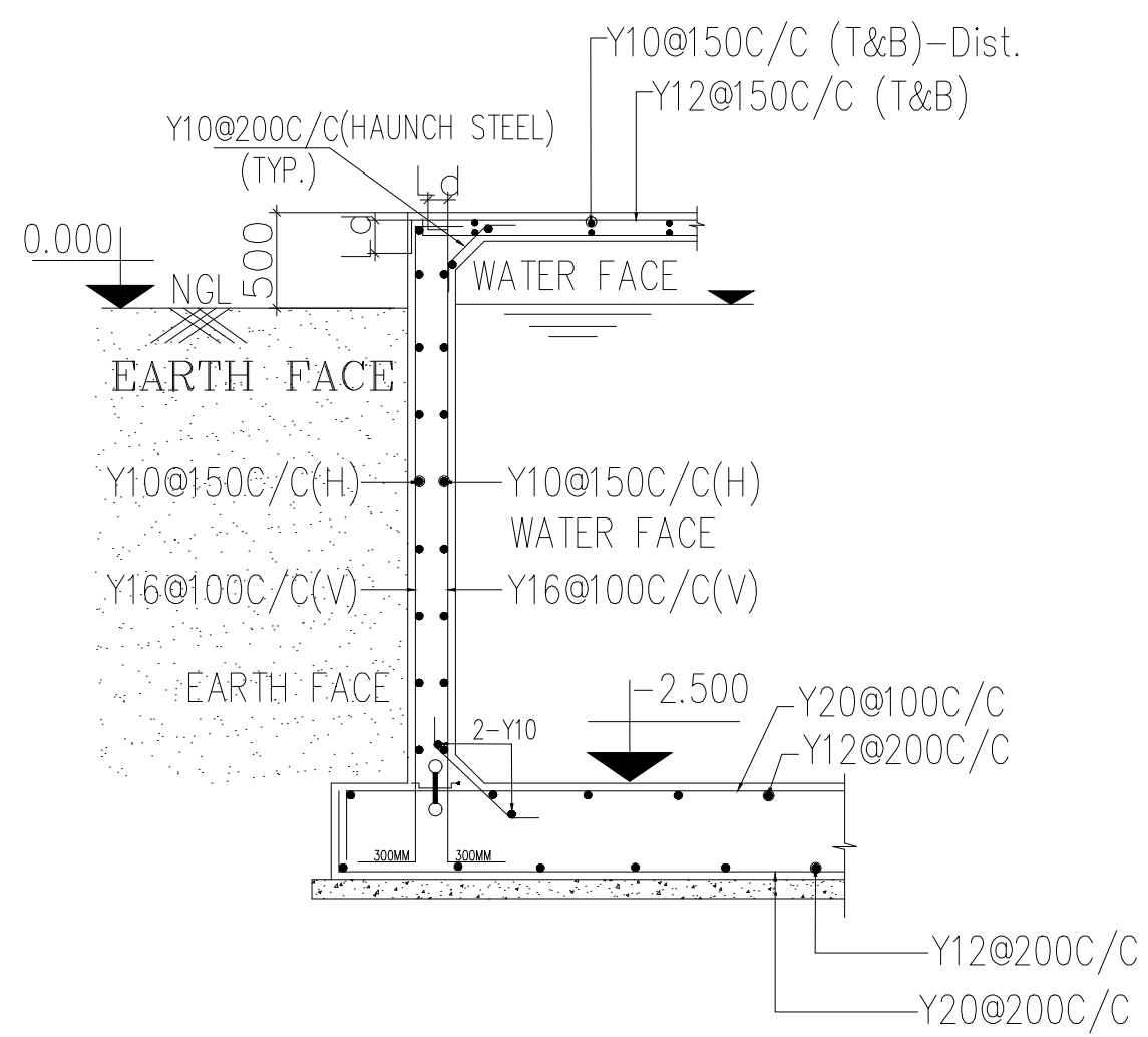
WALL-1 DETAIL SEC-CC REINFORCEMENT DETAIL
