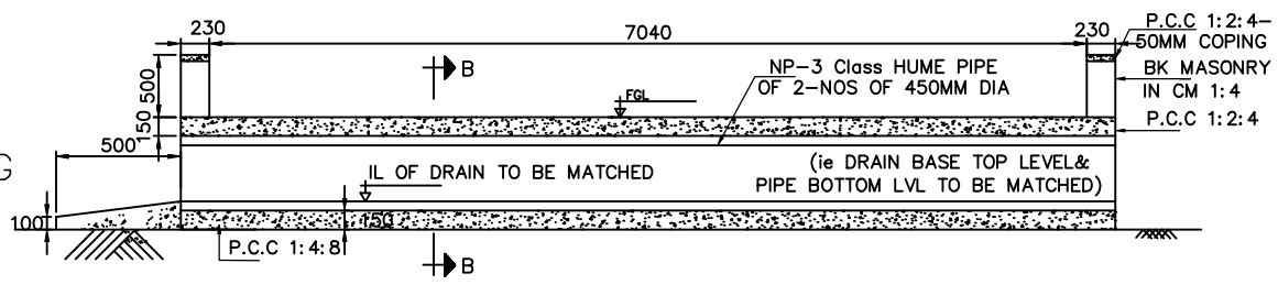
LONGITUDINAL SECTION OF PIPE CULVERT
