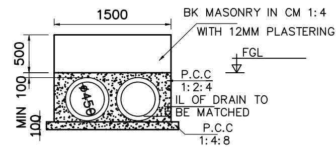
SECTION B-B FOR (PC-1)
