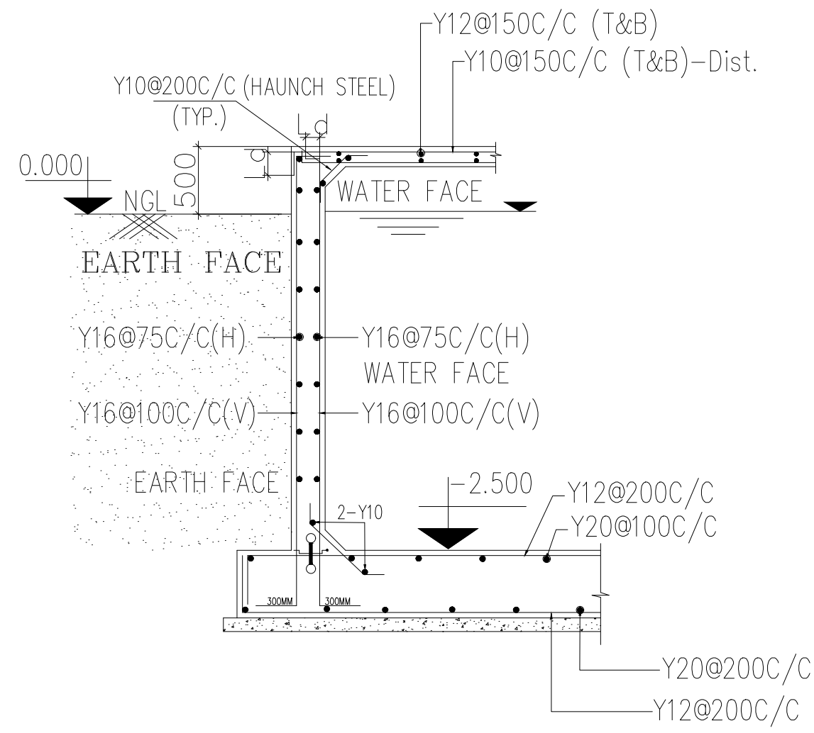
WALL-2 DETAIL SEC-DD REINFORCEMENT DETAIL
