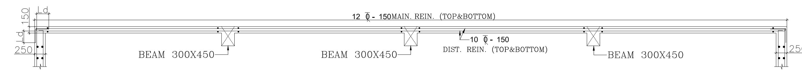
C/S OF ROOF SLAB(150MM THK) DETAIL
