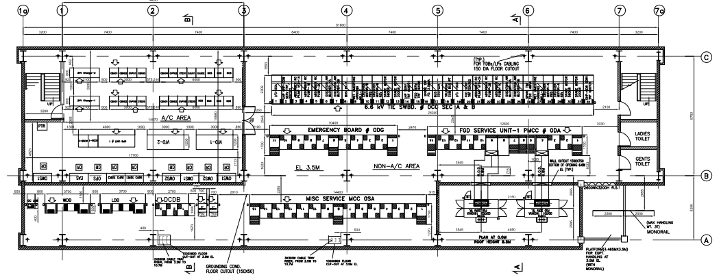
PLAN AT 3.5M
