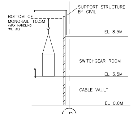
TYPICAL ARRANGEMENT OF EQUIPMENT HANDLING AT EL. 3.5M WITH MONORAIL
