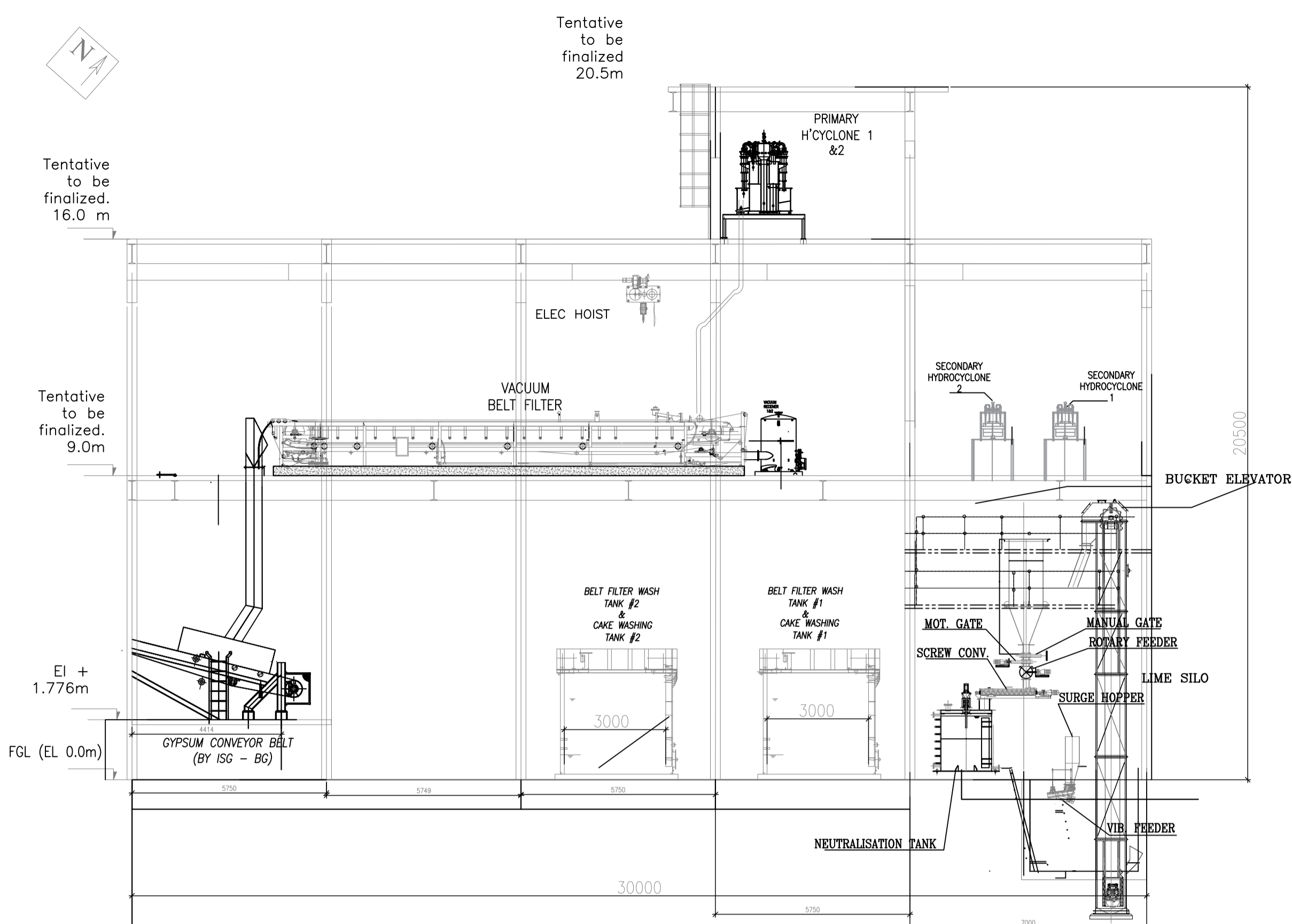
SECTION - BB
