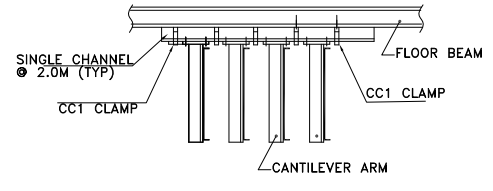
(TYPICAL FIXING DETAILS FOR FIXING OF CROSS TRAYS)
