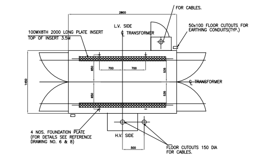
TYPICAL FOUNDATION PLAN FOR DRY TYPE TRANSFORMER
